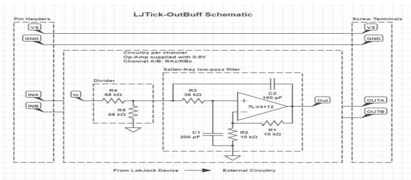
Figure 3: LJTick-OutBuff Schematic
