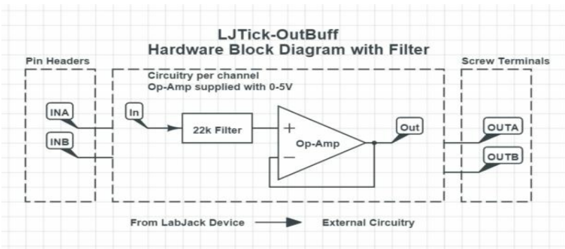
Figure 3: LJTick-OutBuff Hardware Block Diagram with Filter
