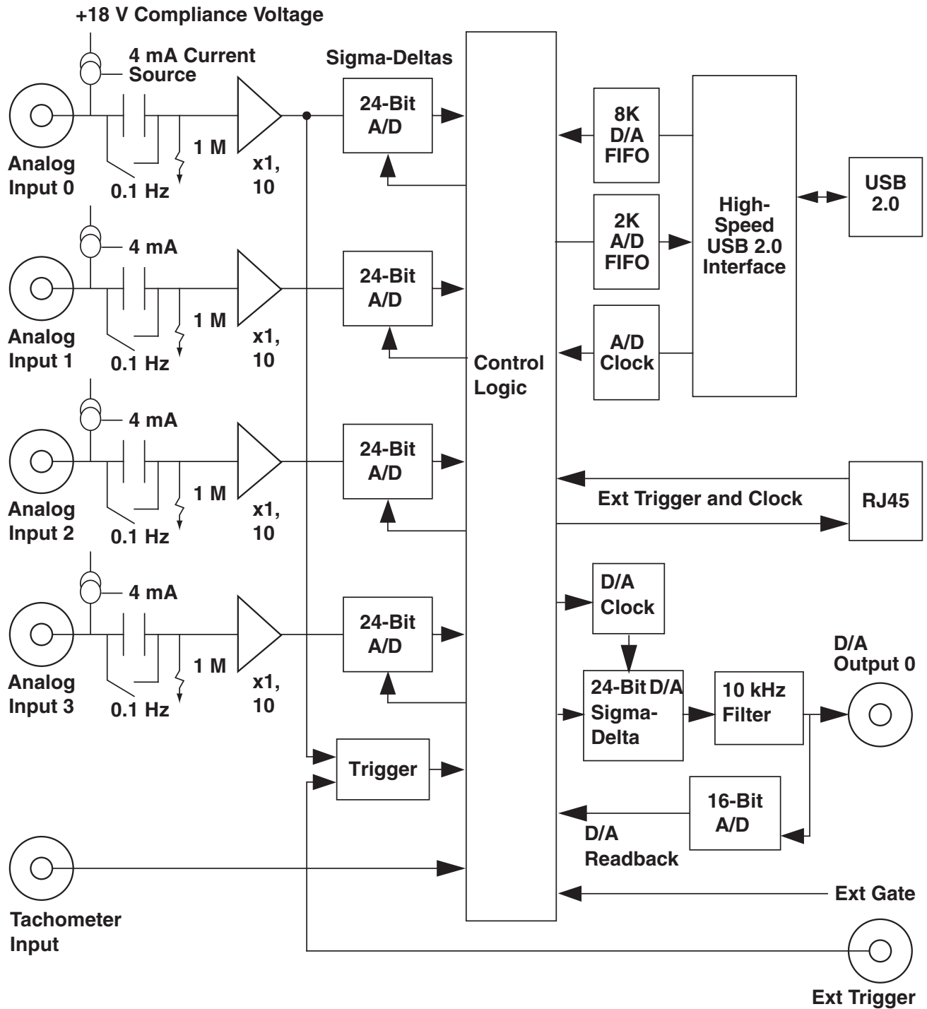
DT9837A Block Diagram
