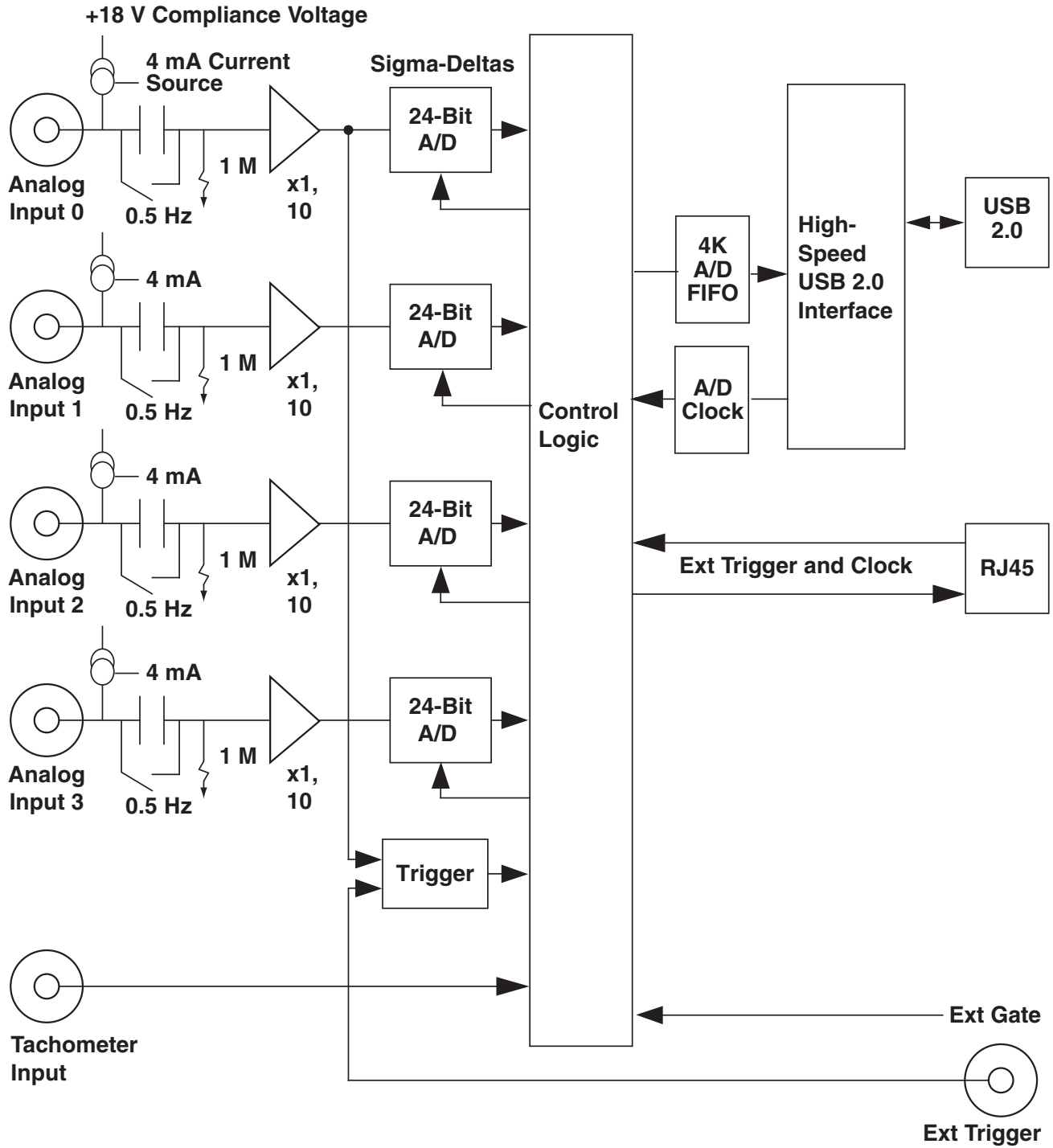
DT9837B Block Diagram
