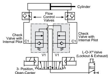
Single, without Trapped Pressure Relief
