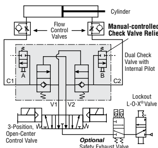
Dual, with Manual Trapped Pressure Relief
