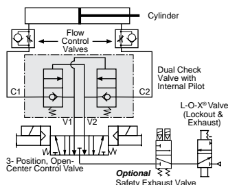
Dual, without Trapped Pressure Relief
