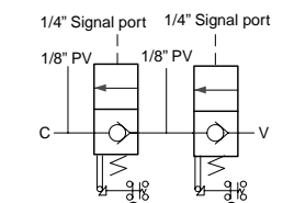
Redundant Pressure Controlled
