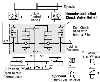
Dual, with Remote Trapped Pressure Relief
