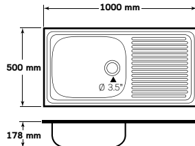
SKS 100 MB, MB/C
