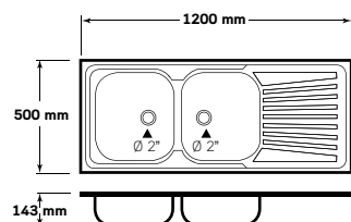
AVP 1206 MA, MA/C
