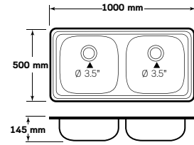
AWC - D 100 MB/C
