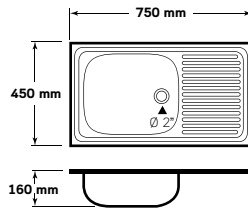
SKS 075 MA, MA/C
