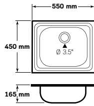
SKS 055 MB, MB/C
