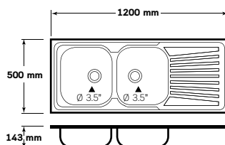
AVP 1206 MB, MB/C
