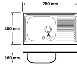
SKS 075 MB, MB/C
