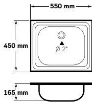
SKS 055 MA, MA/C
