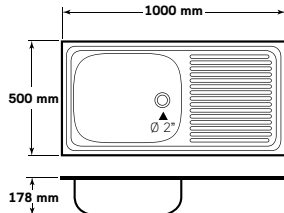
SKS 100 MA, MA/C
