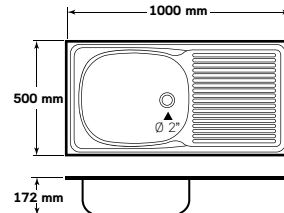
SKA9 100 MA, MA/C
