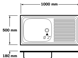
AVP 100 MA, MA/C
