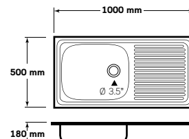
AVP 100 MB, MB/C
