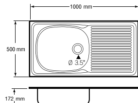
SKA9 100 MB, MB/C
