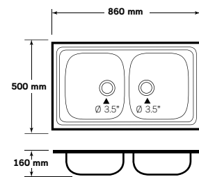
AV-D 086 MB, MB/C
