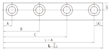
■ Mounting bolt hole : 4
