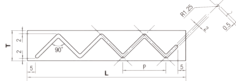
■ Details of Oil Groove
