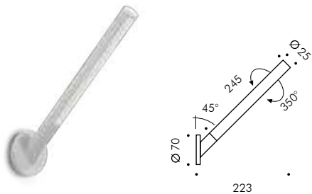
Spillo tilted applique
