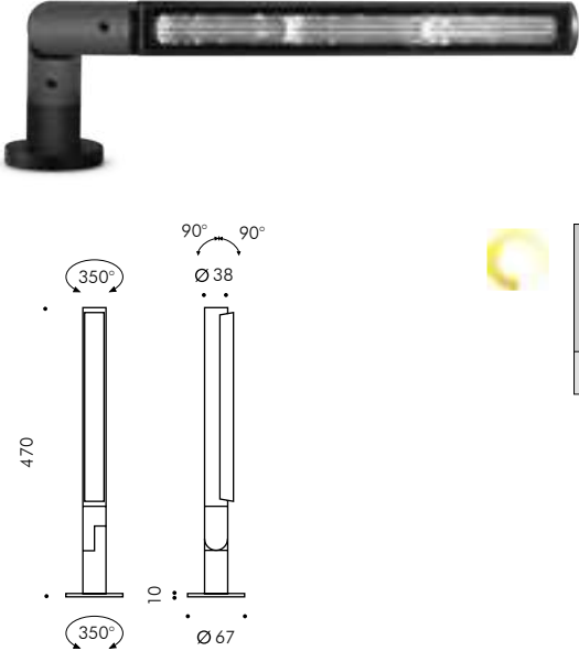
LED TUNABLE WHITE with flat base (24V PWM)
