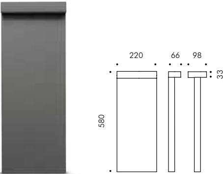
Minilook bollard H 580mm
