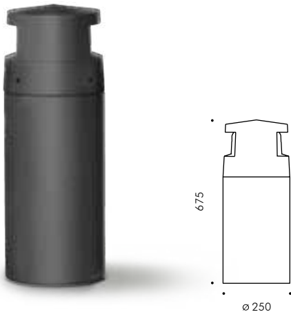
Reef bollard 2 x 90° with reflector
