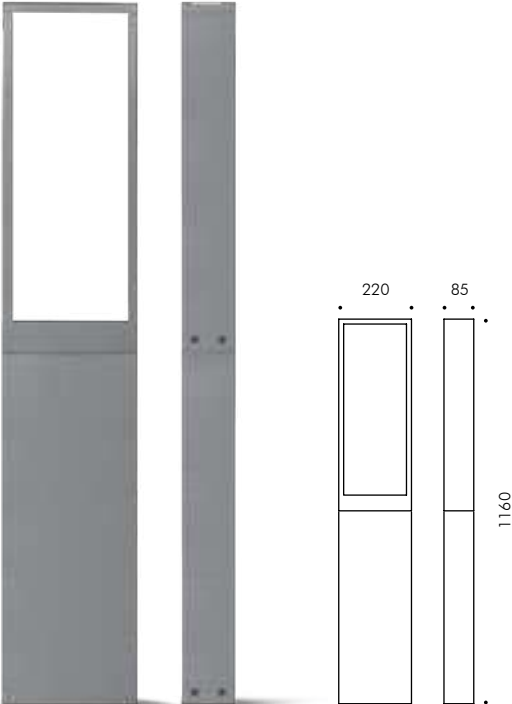
Cool Square long bollard H 1160mm
