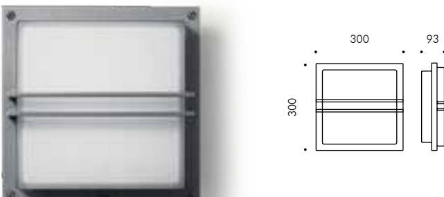
Square 300mm with grille
