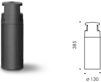
Microreef bollard 2 x 90° with reflector
