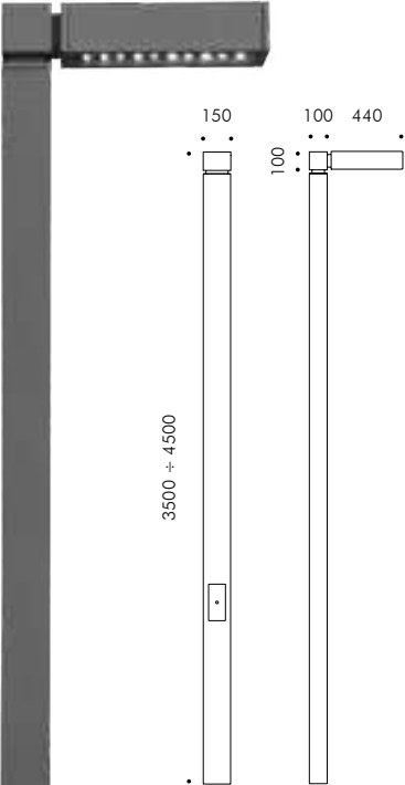
Single 20 LEDs with lenses
