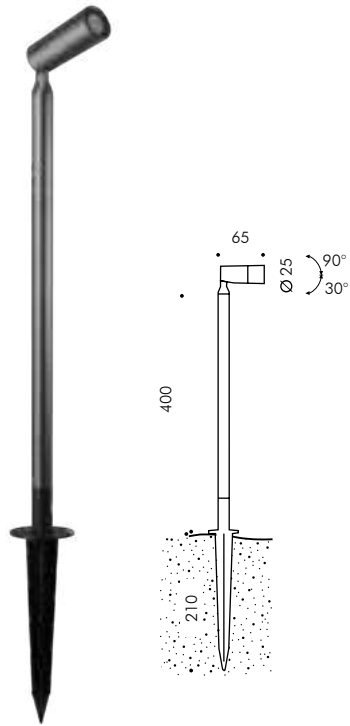
FLOWER 25 bollard including stake
