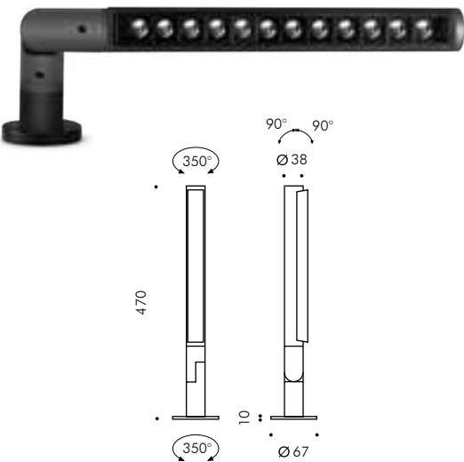
12 LED with flat base (850mA)
