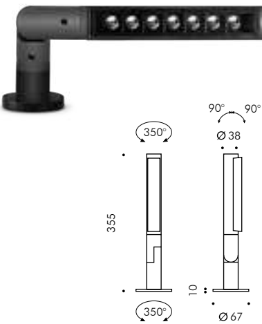
7 LED with flat base (850mA)
