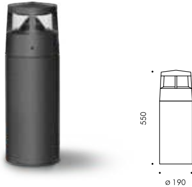
Minireef bollard 360° with reflector
