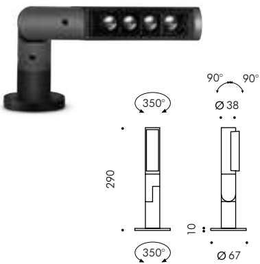
4LED with flat base (850mA)
