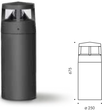
Reef bollard 360° with reflector
