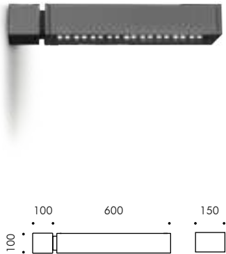
36 LEDs with lenses
