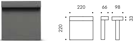
Minilook bollard H 220mm
