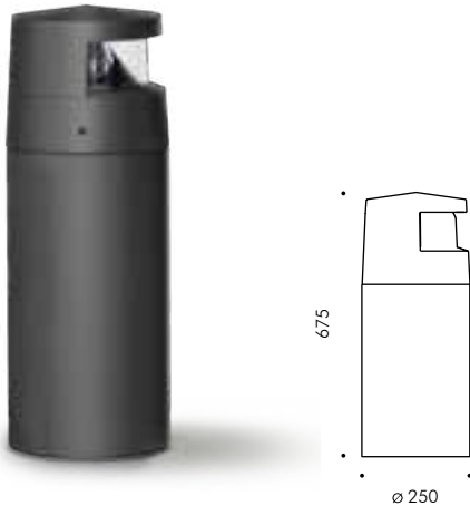
Reef bollard 180° with reflector
