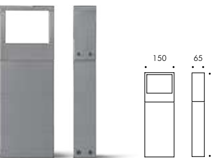
Minicool Square bollard H 450mm
