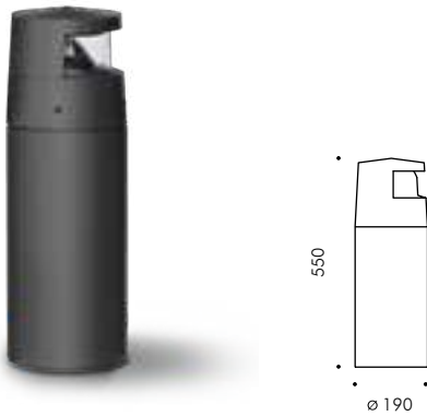
Minireef bollard 2 x 90° with reflector
