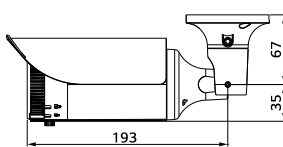
[ LNU3230R_Side / Rear ]
