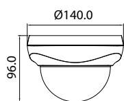
[ LND3230R_Side / Rear ]
