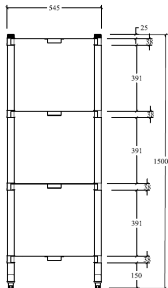
CROSS SECTION
