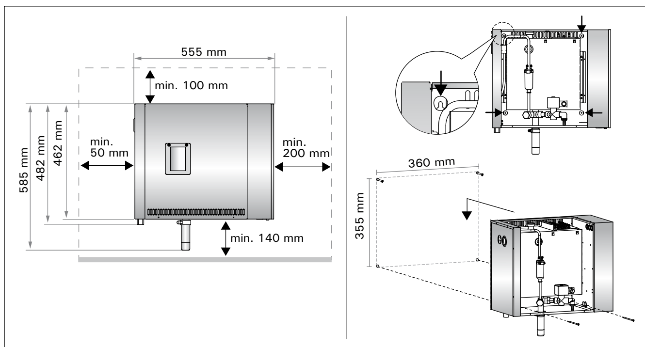
Figure 5. Installation measurements Abbildung 5. Montageabmessungen
