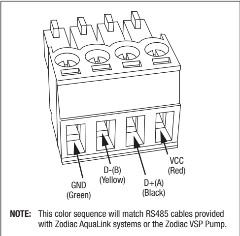
Figure 42. Halo RS485 Connector
