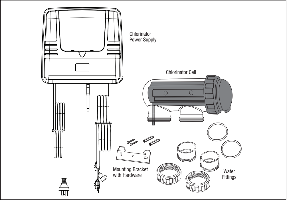
Figure 1. Kit Contents
