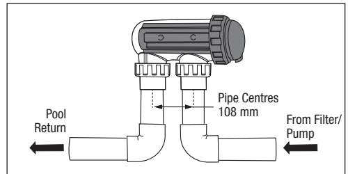
Figure 4. Chlorinator Cell Installation
