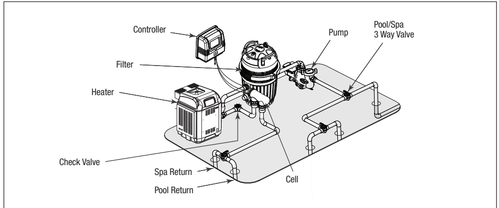
Figure 3. Typical Installation Diagram
