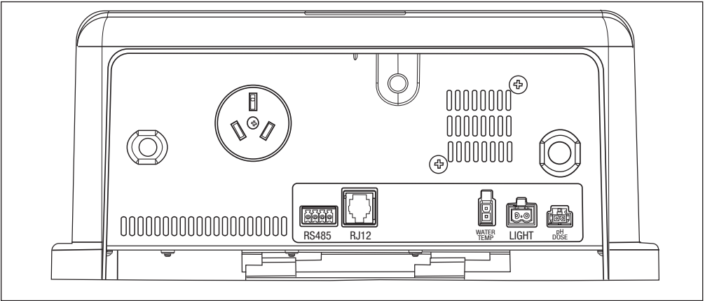
Figure 2. Base View
