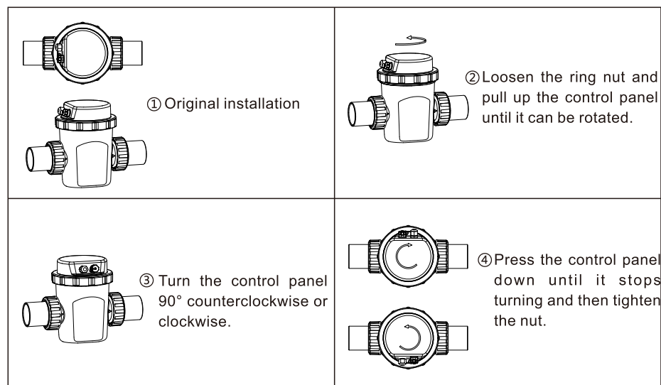
How to adjust the control panel orientation
