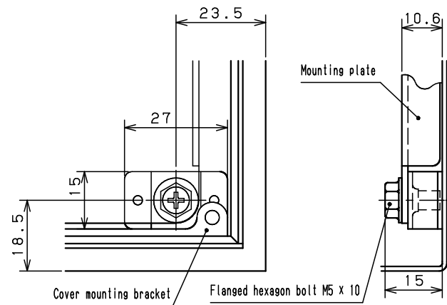
Mounting plate installation B (1:1)
