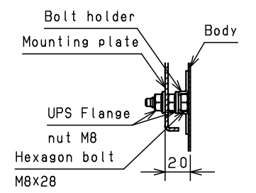
CROSS SECTION B-B 1:3
