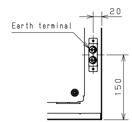
CROSS SECTION C-C 1:5
