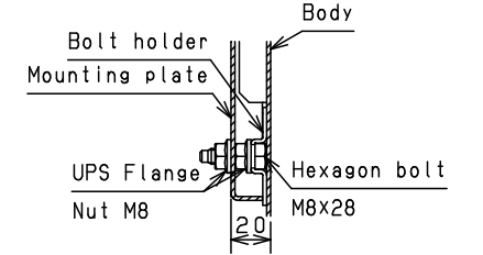
CROSS SECTION B-B 1:3
