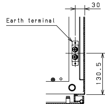
CROSS SECTION C-C 1:5
