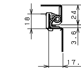
CROSS SECTION B-B 1:2
