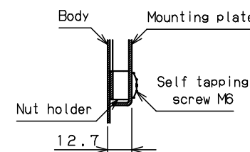
CROSS SECTION C-C 1:2
