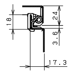
CROSS SECTION B-B 1:2
