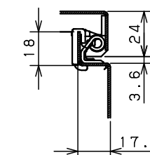
CROSS SECTION B-B 1:2
