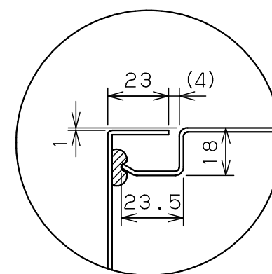
Cross section A (1:2)
