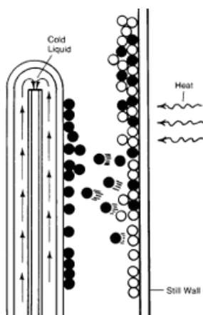
Wiped-Film still technology
