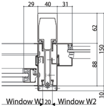
Mullion 180 C Type
