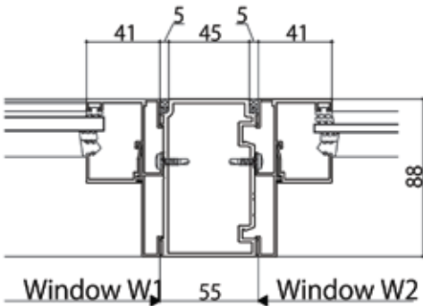
Reinforcement Mullion 180
