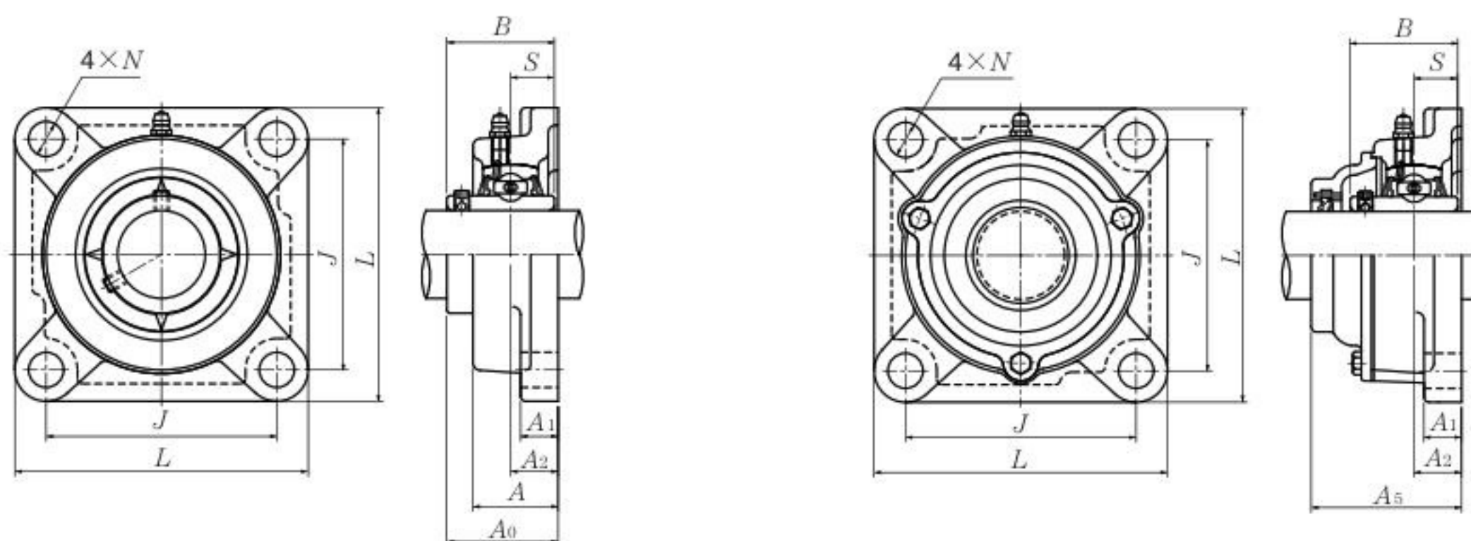
Cast dust cover type (Open end) C-UCF...D1
