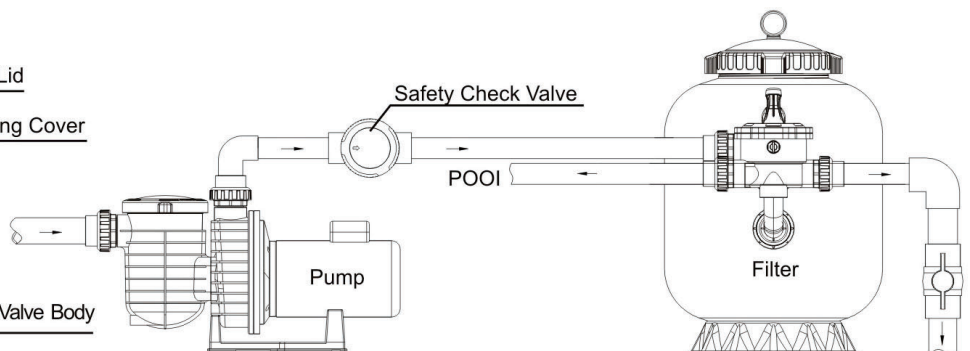
WL-DZF Series Exploded Drawing And Installation Diagram
