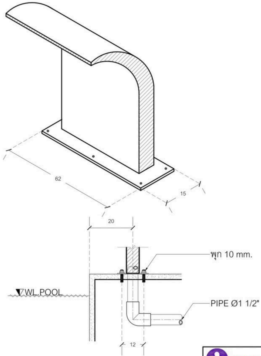
DETAIL WATER CURTAIN PSW-22 SCALE 1 : 10
