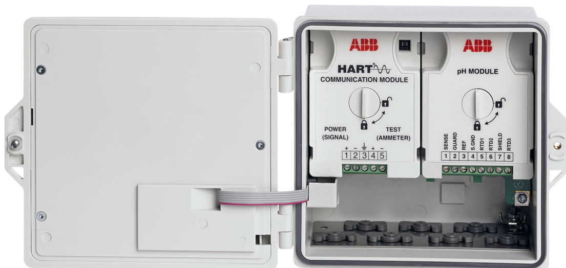
Figure 2 AWT210 communication/sensor modules
