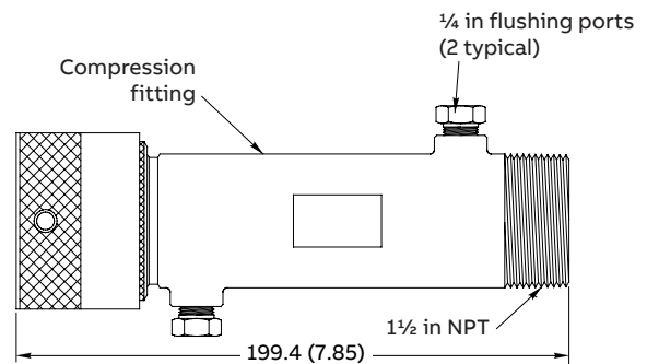
Hand-tight
