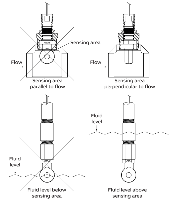
Figure 10 Installation
