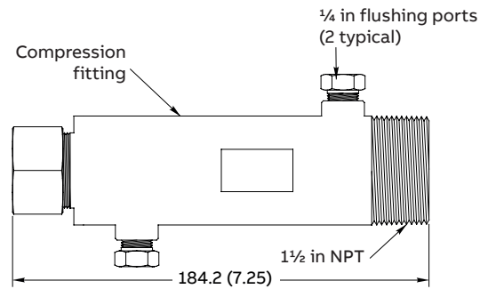
Wrench-tight
