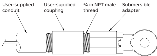
Figure 8 TB404 sensor with submersion assembly
