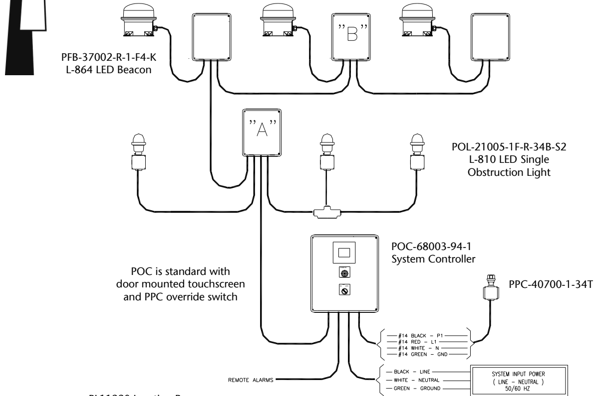
PL11220 Junction Box
