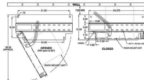
Swing Racks
