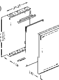
BWM-9312-1600 Fan Assembly (2) 4" (0.10 m) Diameter Fans (160 CFM) w/Guard
