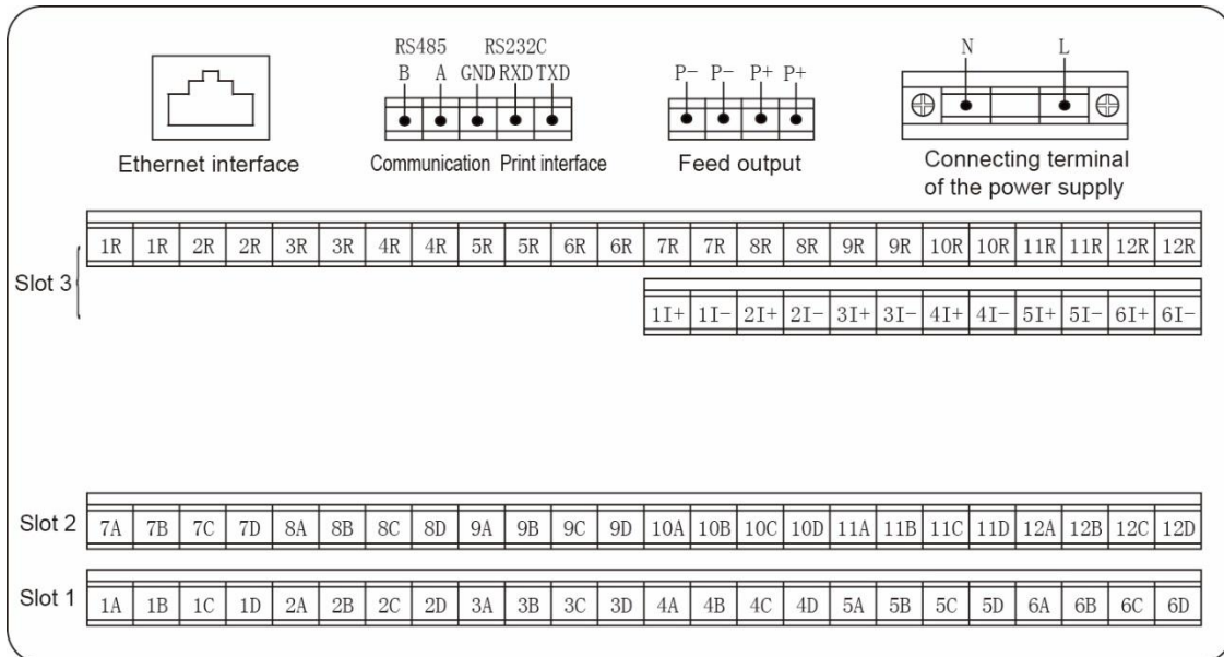
Terminal diagram of instrument tail
