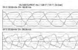
<Before installing APF>
