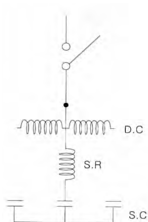
⟨Discharge coil with internal reactor⟩
