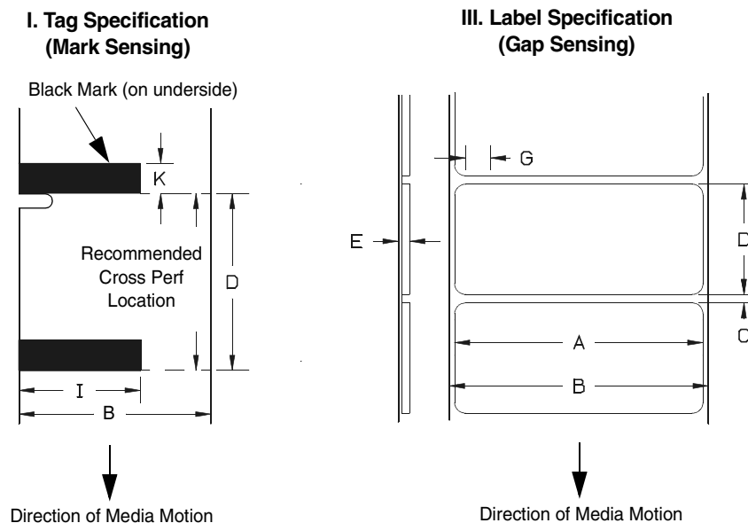
Figure 5. Media Dimensions
