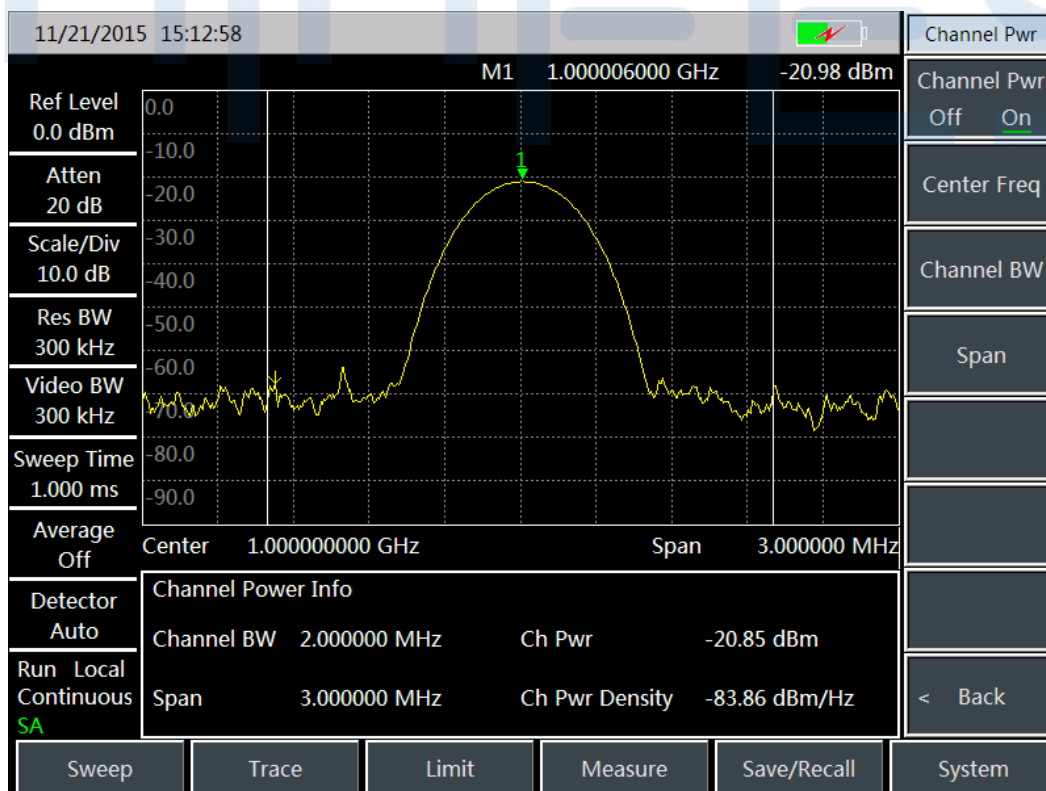
Channel Power
