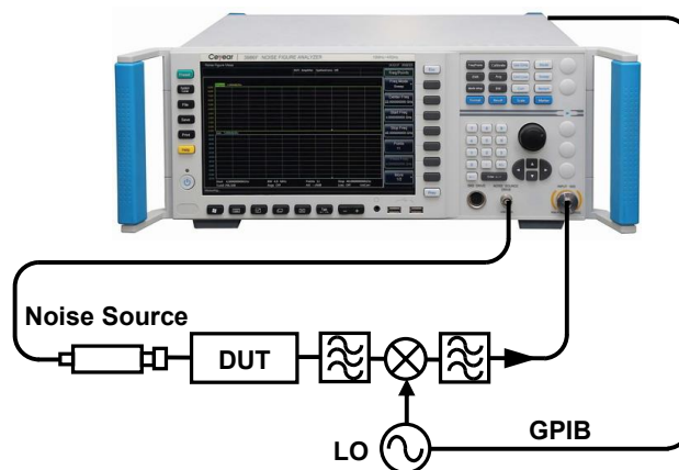
Measurement Setup
