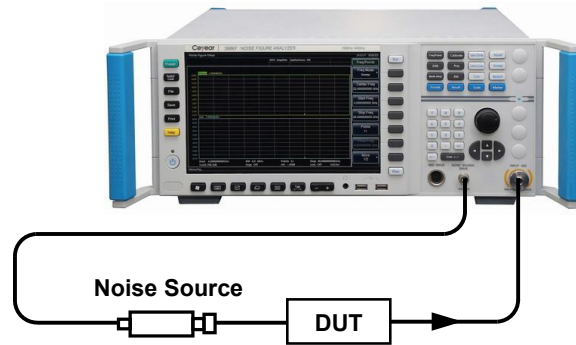
Measurement Setup
