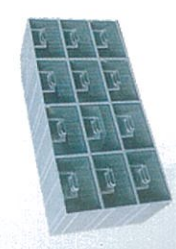
Model : 002-9 Ext. Size : 170 x 456 x 220 MM. Chs. Size : 170 x 115 x 73 MM. Chs. Q'ty : 12
