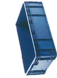
Model : 031/1031/131-I Ext. Size : 293 x 379 x 134 MM. Int. Size : 260 x 344 x 123 MM.
