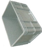
Model : 331.5 Ext. Size : 335 x 335 x 149 MM. Int. Size : 330 x 300 x 136 MM.
