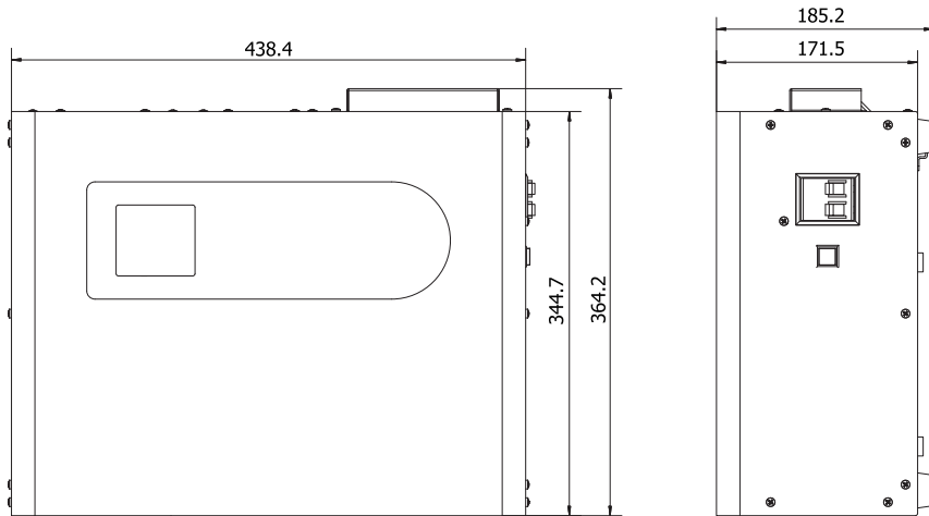
MST-10KVA
