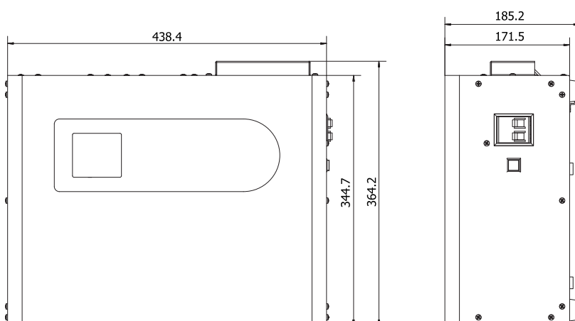
MST-10KVA
