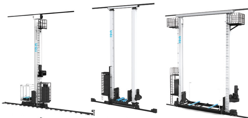
WALI STACKER CRANE MOBILE ROBOT C-50L/C-1200S/C-1200L/C-3000
