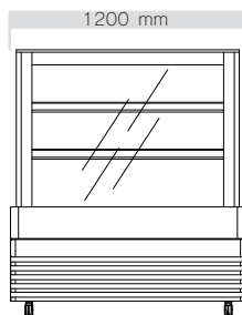
FRONT VIEW : SQRCD-12
