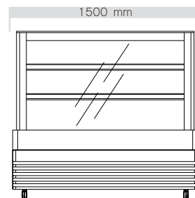
FRONT VIEW : SQRCD-15
