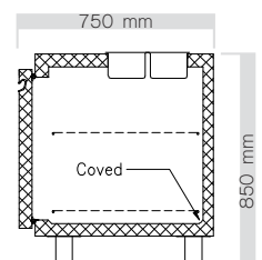
SECTION SIDE VIEW
