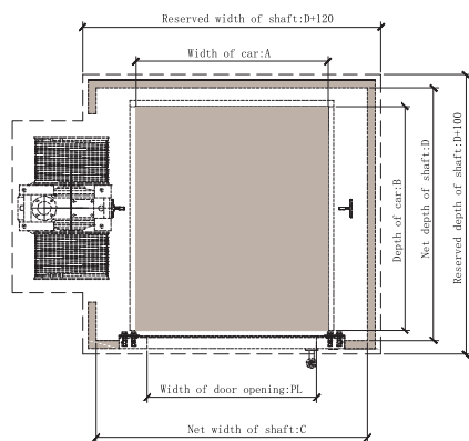
Floor plan of down-mounted shaft
