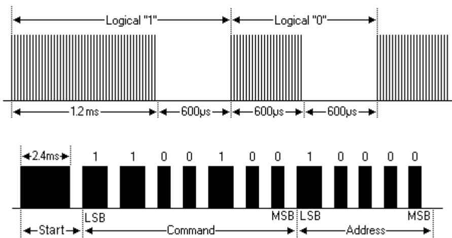
Waveform Infrared Remote
