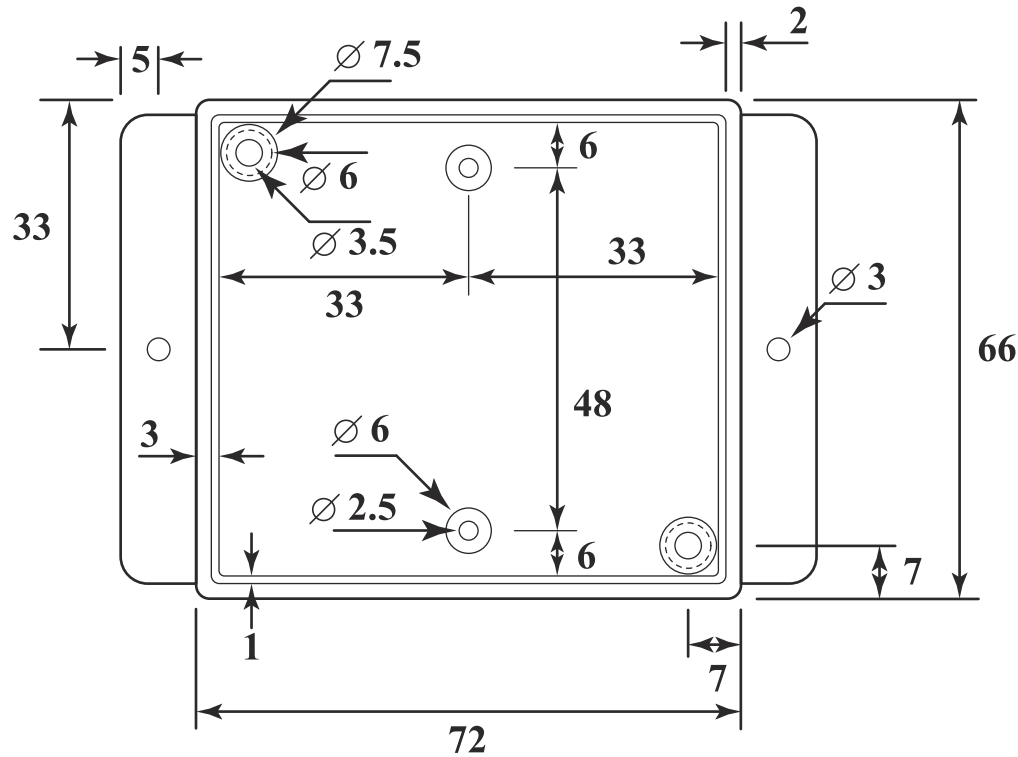
Bottom View
