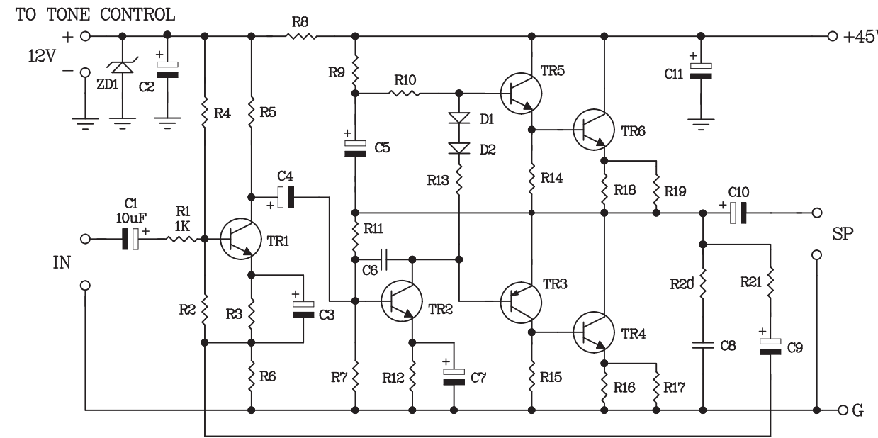
Figure 1. The Power Amp OTL 30W R1% Circuit
