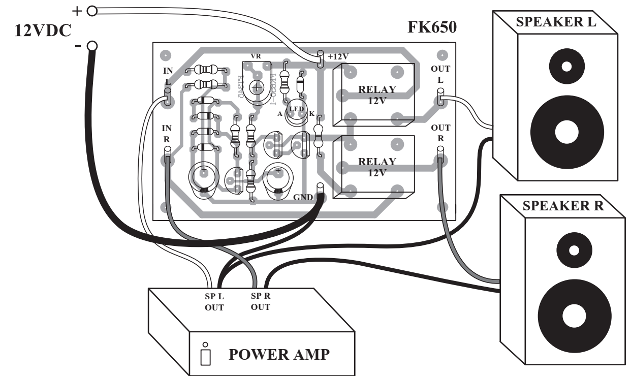
Figure 2. Circuit Assembling
