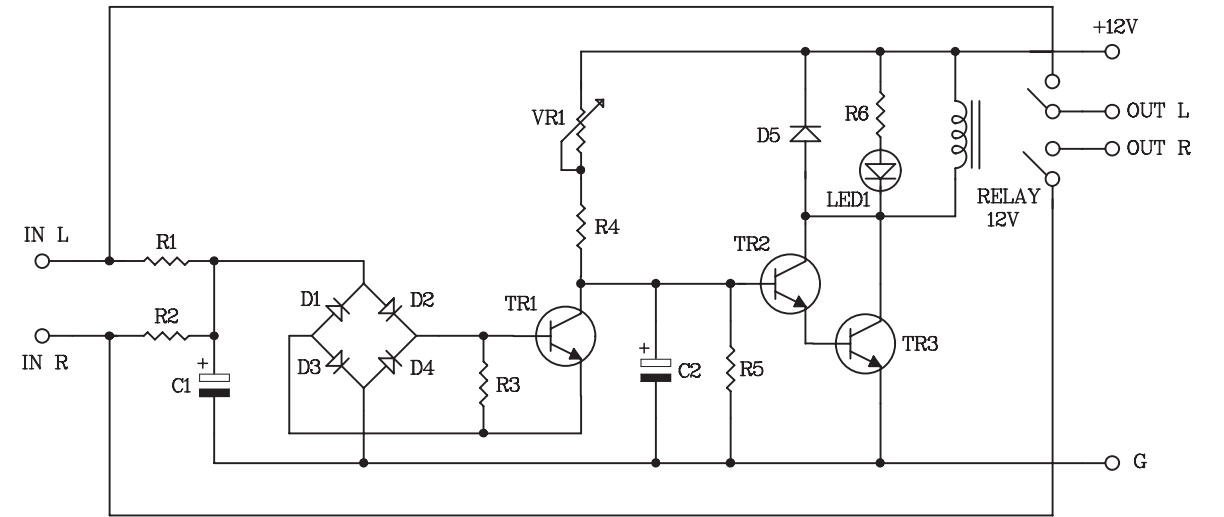
Figure 1. The Speaker Protection (Stereo) Circuit
