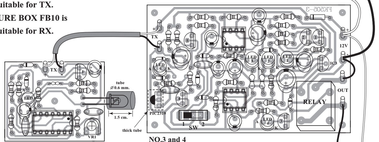
Figure 2. Circuit Assembling
