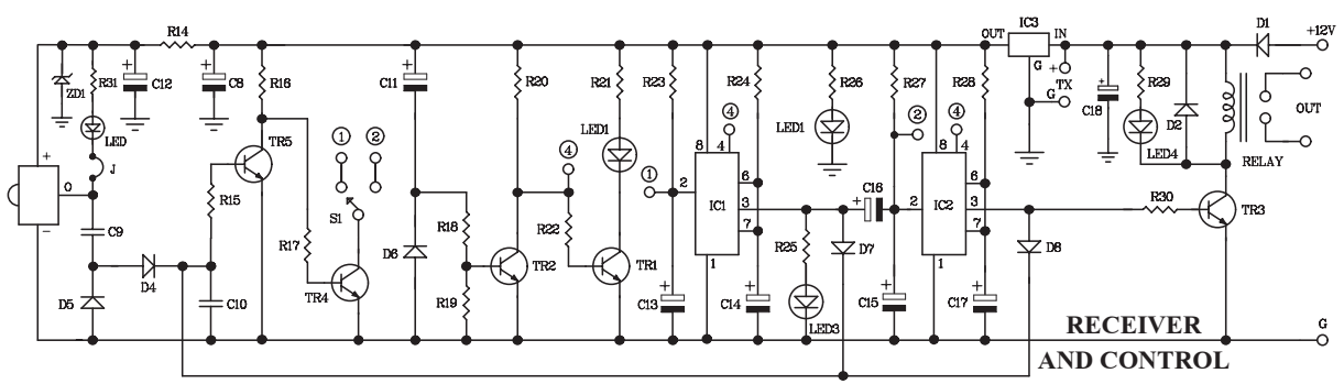
Figure 2. Circuit Assembling
