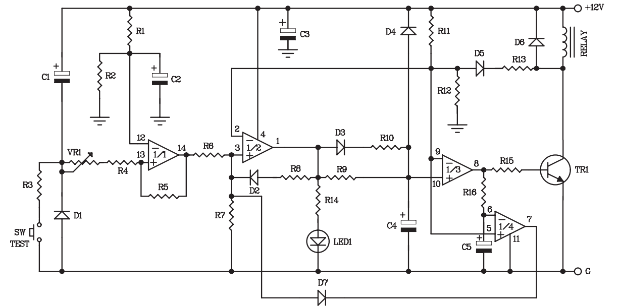
Figure 1. Car Starting Alarm Circuit
