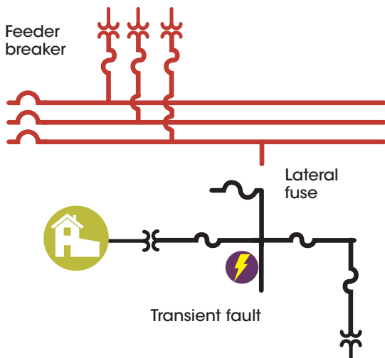
Figure 1. "Fuse-blowing" philosophy.
