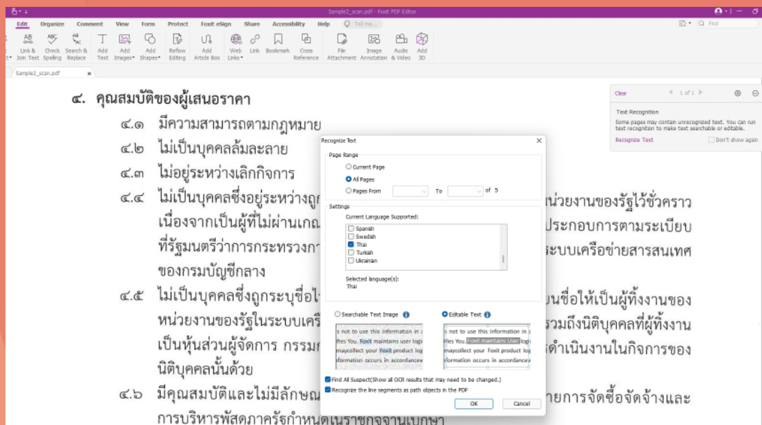
Before OCR
