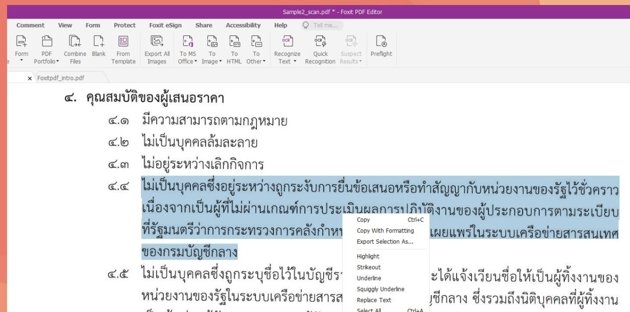
After OCR
