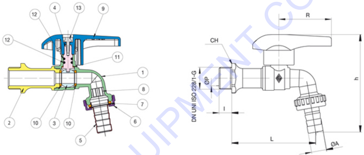
Hose ball bib-cock with hose tail connection and aluminum handle
